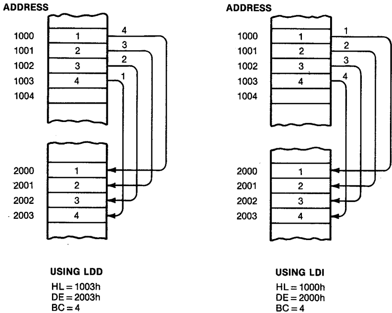
Fig. 13-1. Transferring a block of memory with nonoverlapping ranges.
